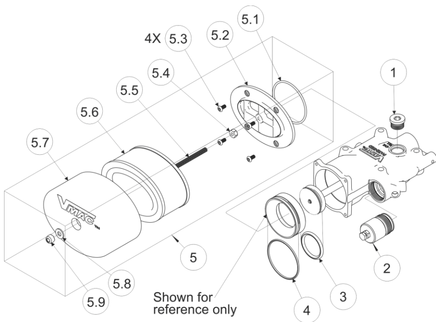
Figure 4 – Inlet Valve Sub Components
