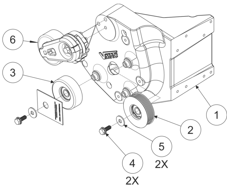
Figure 5 – Main Bracket Assembly
