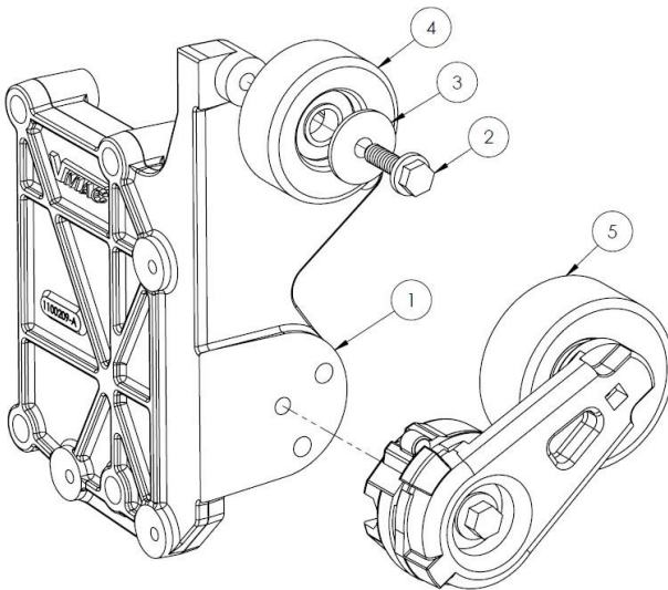
Figure 5 - Main Bracket Assembly
