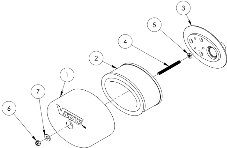
Figure 8 – Air Filter Assembly
