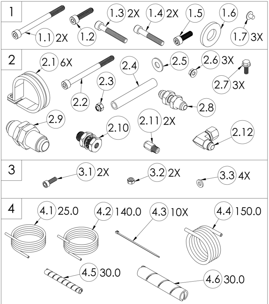
Figure 2 - Fastener Pack
