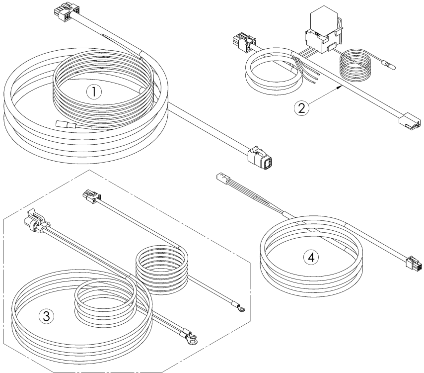
Figure 9 – Electrical Pack
