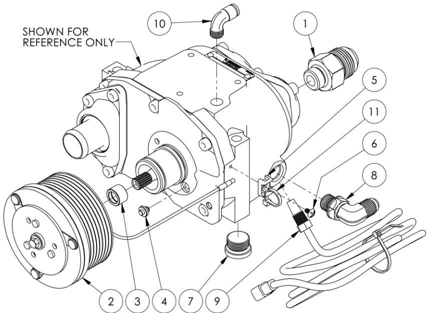
Figure 4 - Compressor Assembly
