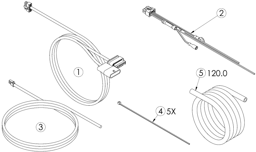
Figure 10 – Electrical Pack
