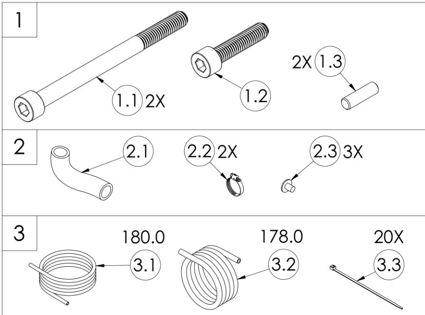
Figure 2 – Fastener Pack
