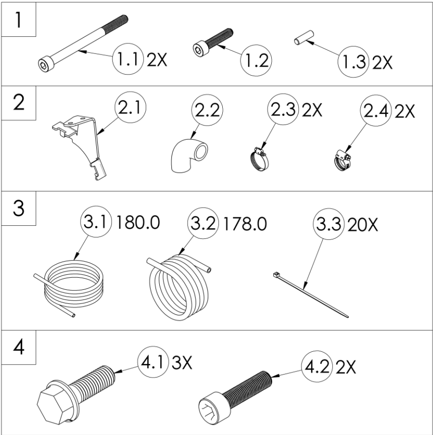
Figure 2 – Fastener Pack
