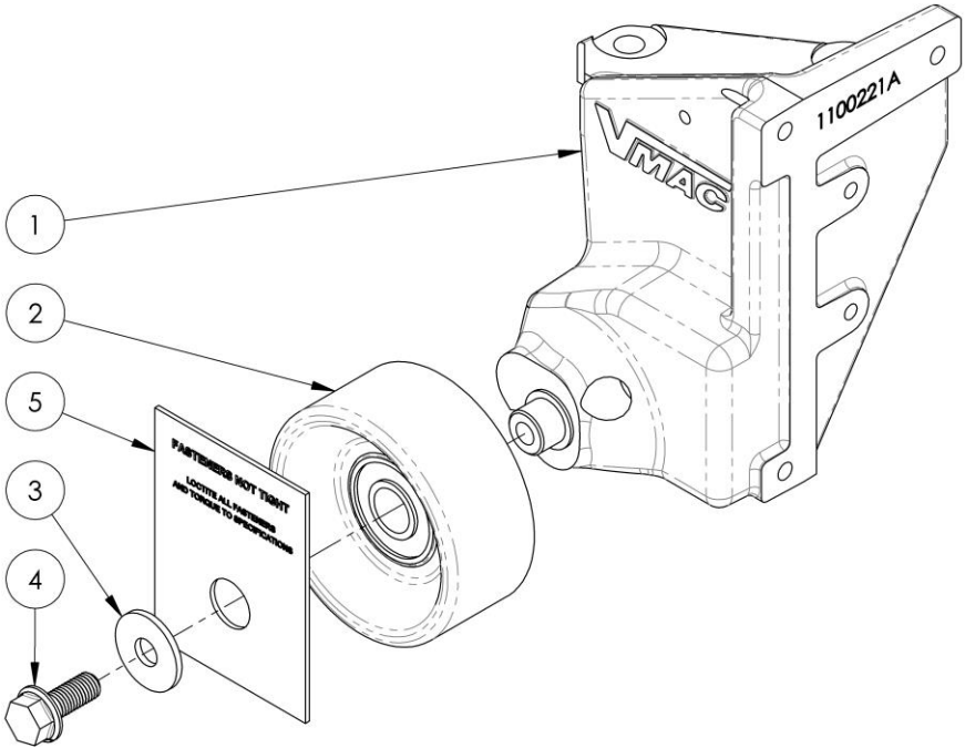
Figure 4 – Main Bracket Assembly
