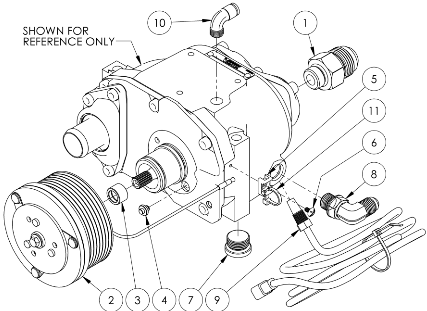
Figure 3 - Compressor Assembly
