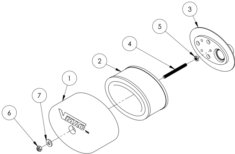
Figure 7 – Air Filter Assembly
