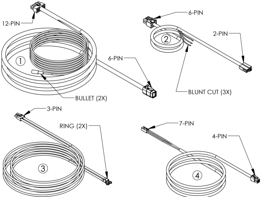
FIGURE 8 – Wire Harness Identification
